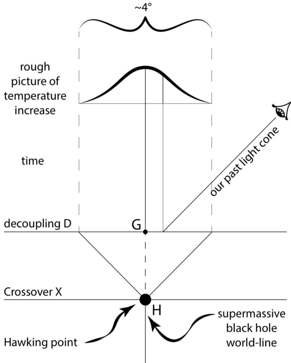
Figure 1 as given in [4] which has competing black hole radiation, and can we see this today in the CMBR?
