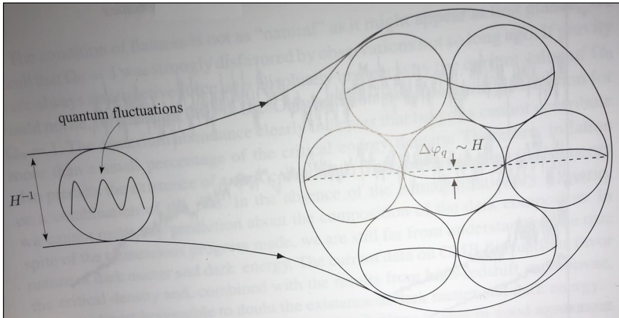
Figure 2 which is from reference [11] , [15]
